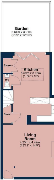
Ground Floor Approx. 40.8 sq. metres (439.4 sq. feet) (excluding Store, Garden)
